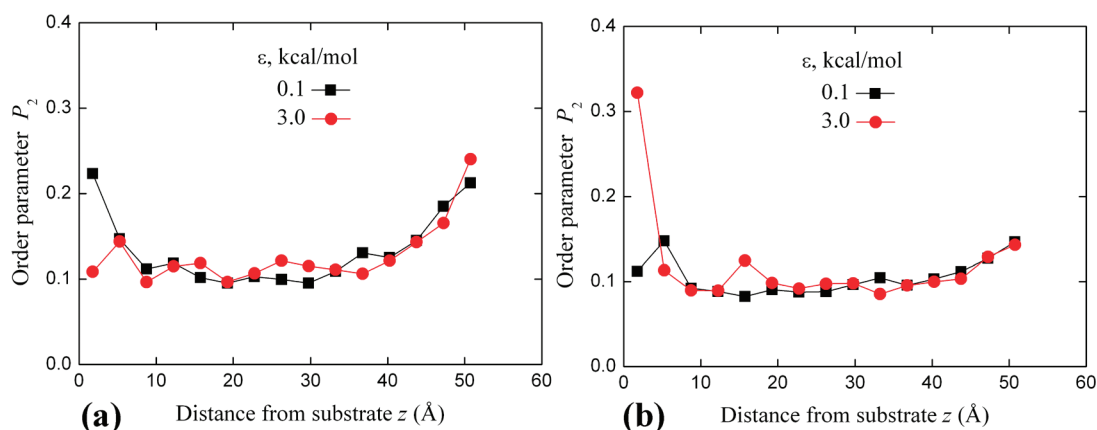
Figure 4. Order parameter P_2 for the aPS backbone vector \bar{v}_{bb} (a), and for the phenyl-ring vector \bar{v}_{ph} (b), for a 16-chains film at T = 540 K and for different strengths of the attraction to the substrate.
