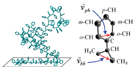
Figure 3. Left: typical snapshot of one aPS chain in a many-chain supported film close to the substrate at T = 540 K and \varepsilon = 3.0 kcal/mol. Right: the aPS monomer with the naming convention of the united atoms, shown together with two vectors, \vec{v}_{ph} for the phenyl ring and \vec{v}_{bb} for the backbone orientation, that are chosen to measure the order parameter P_2 . Here o = ortho, m = meta, and p = para.
