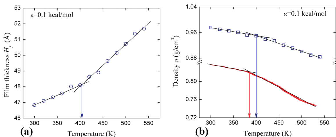
Figure 7. Film thickness (a) and average film density (b) as a function of temperature for aPS film with 16 chains in the case of a weak attraction ( \varepsilon = 0.1 kcal/mol) to the substrate. The circles represent the thickness H_f of the whole film using the GDS. The squares represent the average density over the whole film, where the thickness of the film is measured as the distance from the substrate to the GDS. The red solid line represents the average density over the whole film, where the thickness of a film is calculated as the distance from the substrate to the maximal value H_{\max} of all z coordinates.
